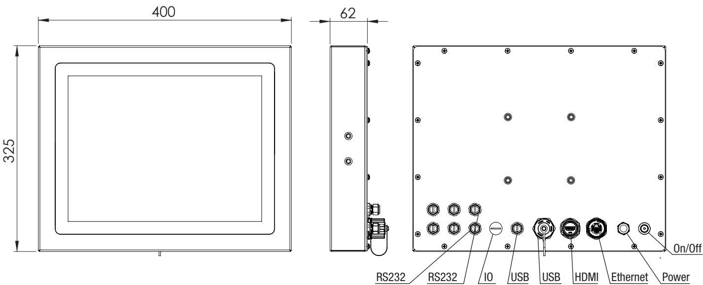
PX15 Housing
