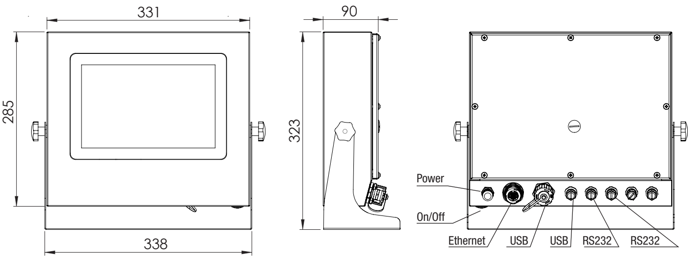
PX10 Housing
