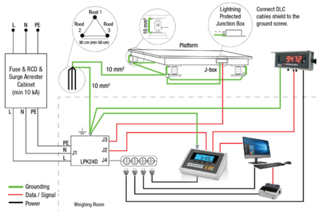
With a dedicated grounding system, cable connection of a scale with digital load cells
